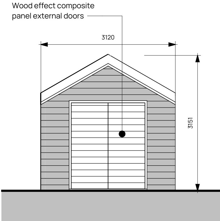
Bin Store Front Elevation 1: 50
