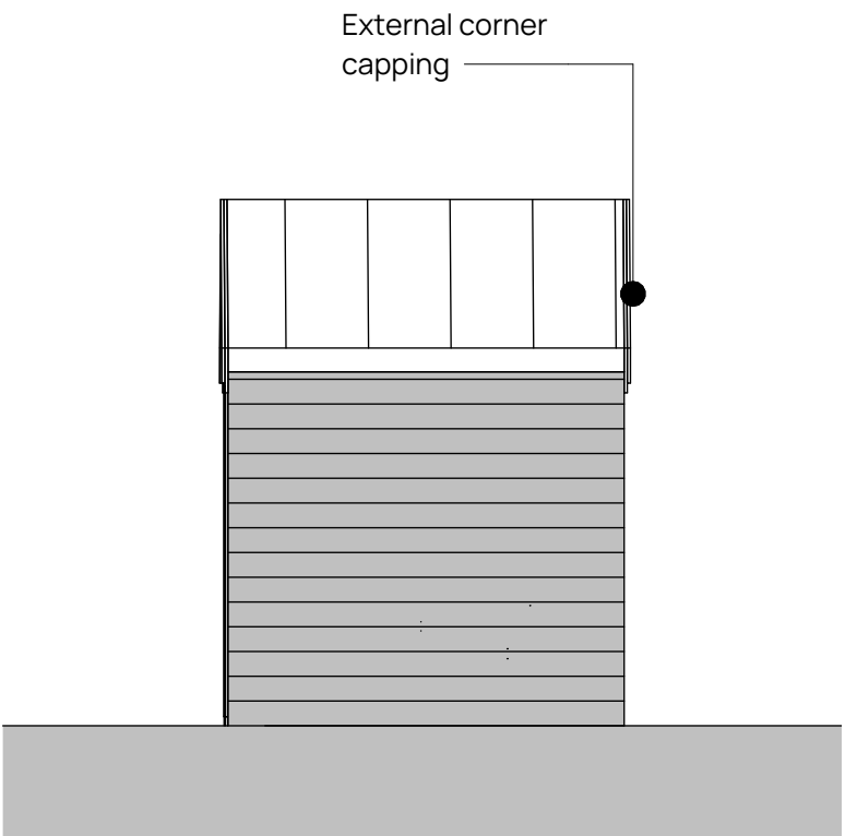
Bin Store Side Elevation 02 1: 50
